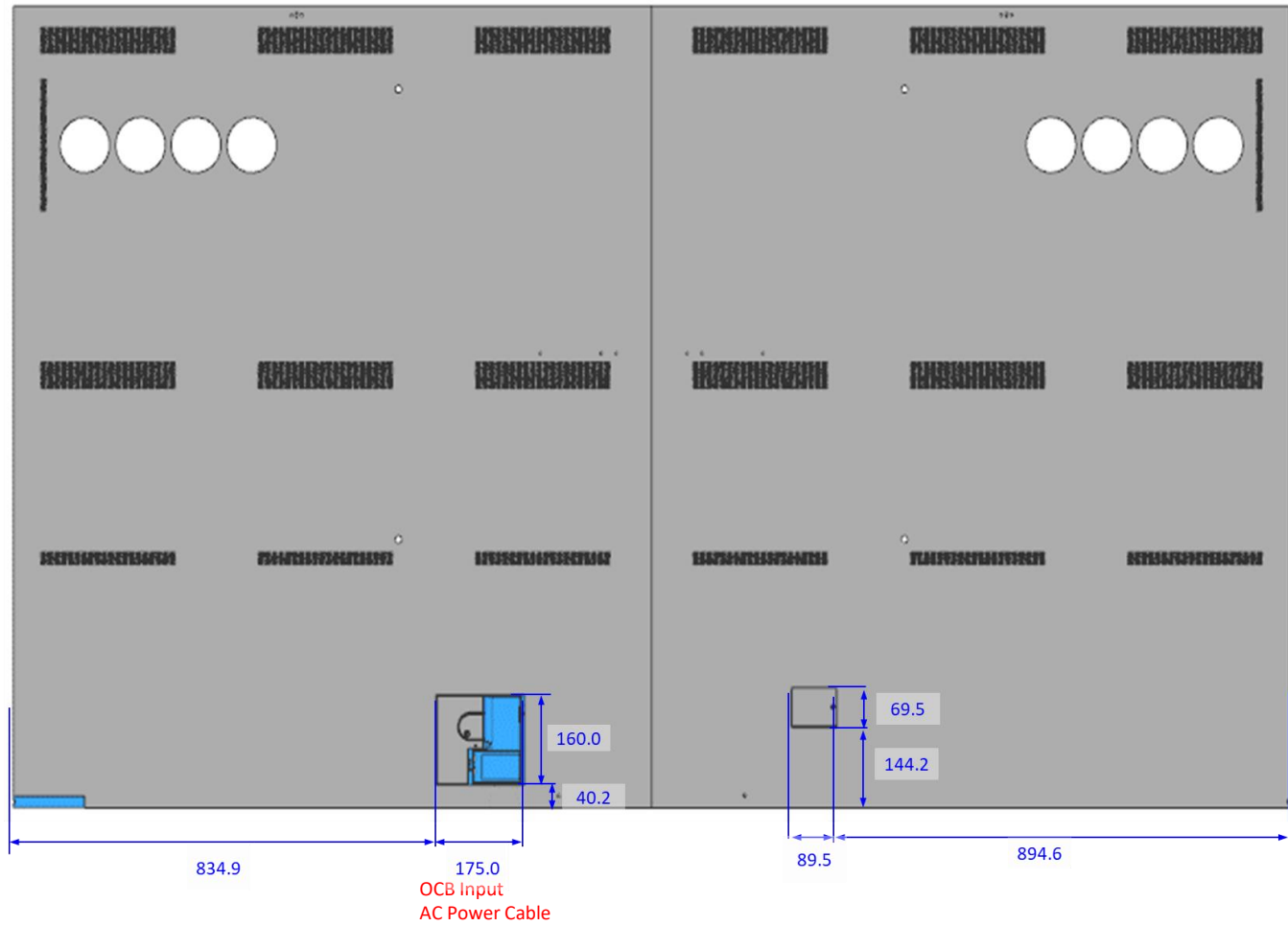
114" Micro LED Cover and Rear-View Dimension
